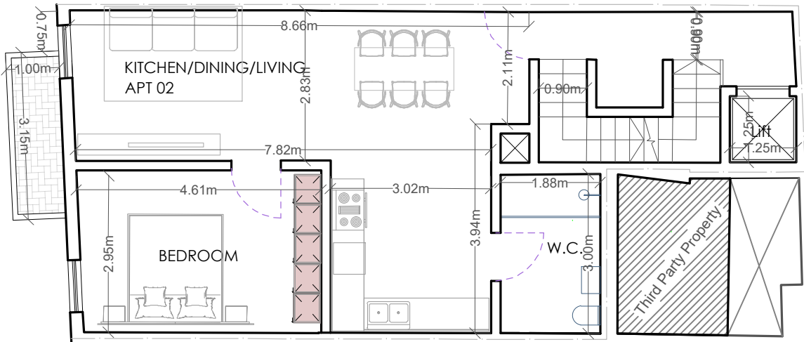
PROPOSED SECOND FLOOR PLAN SCALE 1:100
